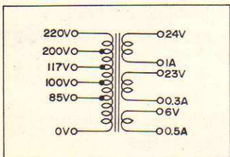
TEAC A-2070/A-2080 TAPE TRANSPORT
